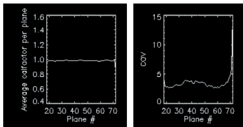
Figure 1 Example of plane average SUV and plane by plane COV (%) analysis of the calibration QC reconstructions
