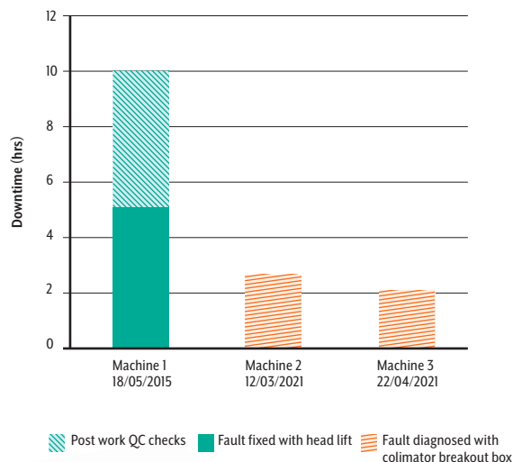
Figure 1 Reduction in downtime using breakout box
