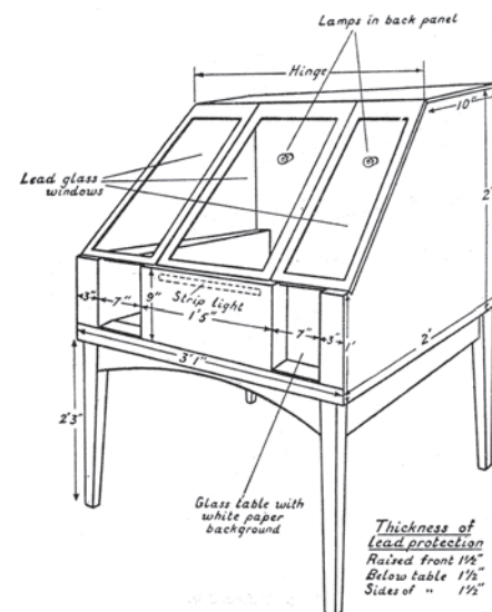
Figure ❶ Design for a radium bench. Radium Commission 3rd Annual Report 1931-1932.
