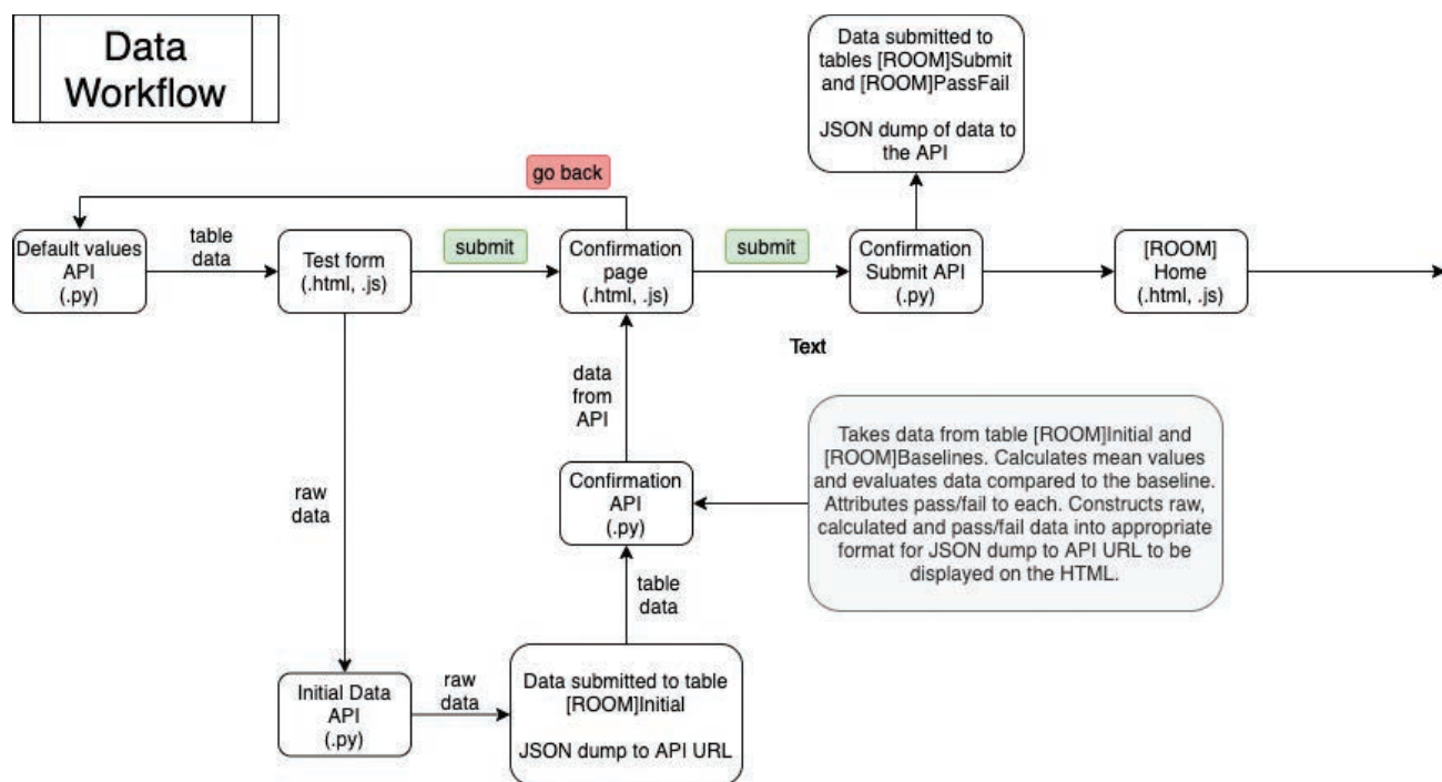
Figure 1 The data workflow for QA data entry. The platform uses a series of application programming interfaces (APIs) to handle the data and display in HTML format.
